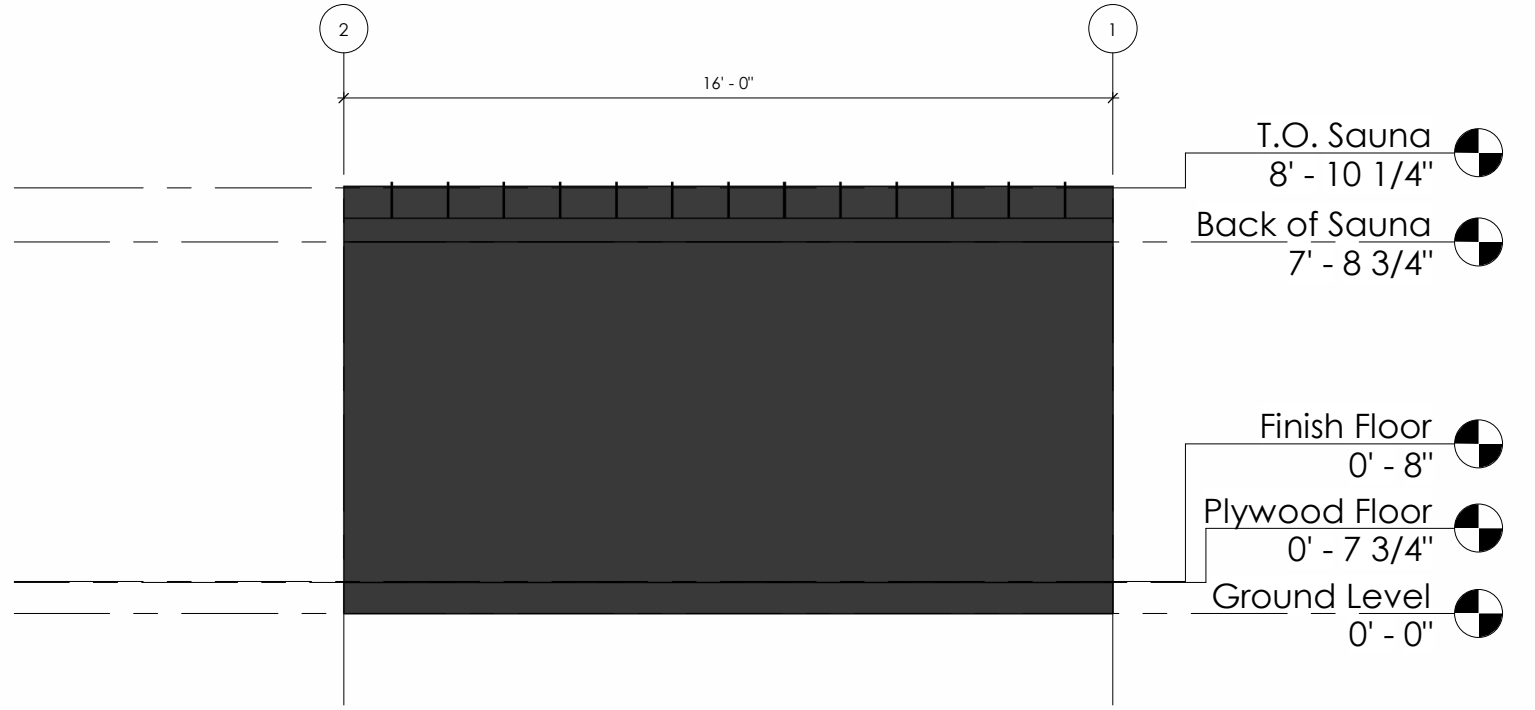
② Back 1/4" = 1'-0"
