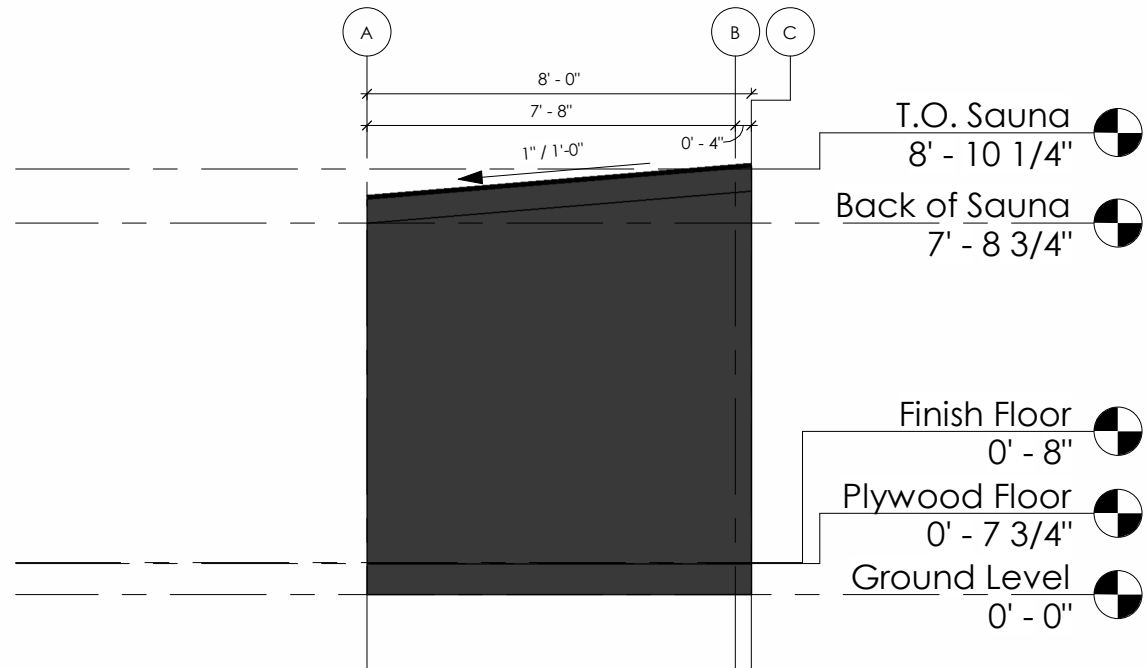
③ Left 1/4" = 1'-0"
