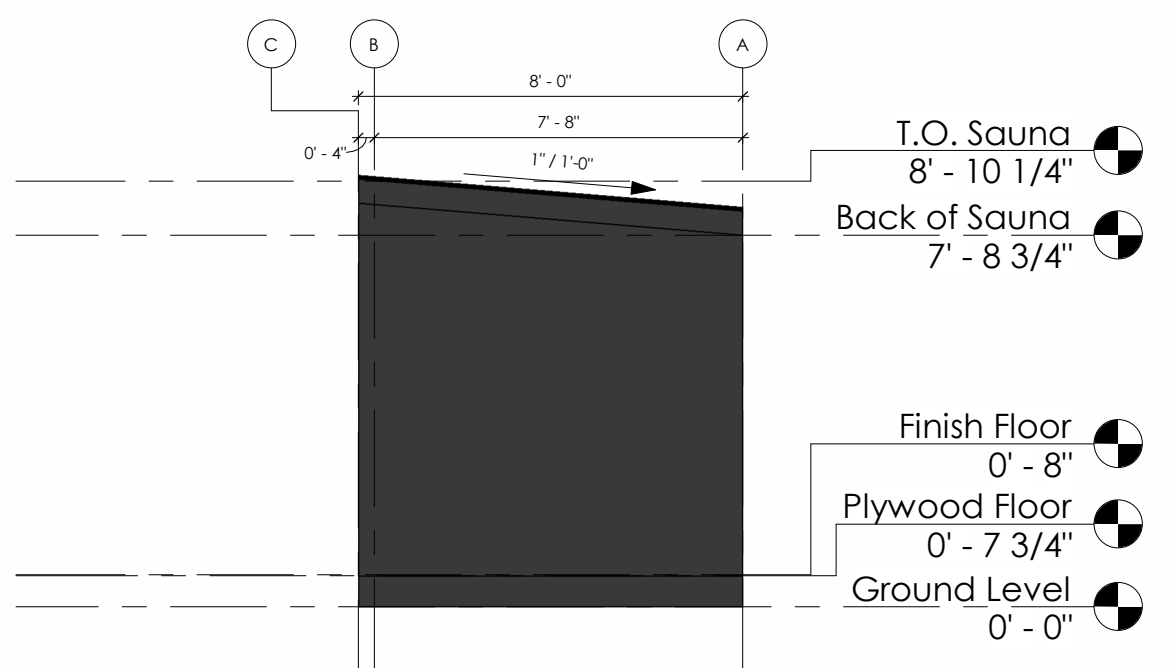
④ Right 1/4" = 1'-0"
